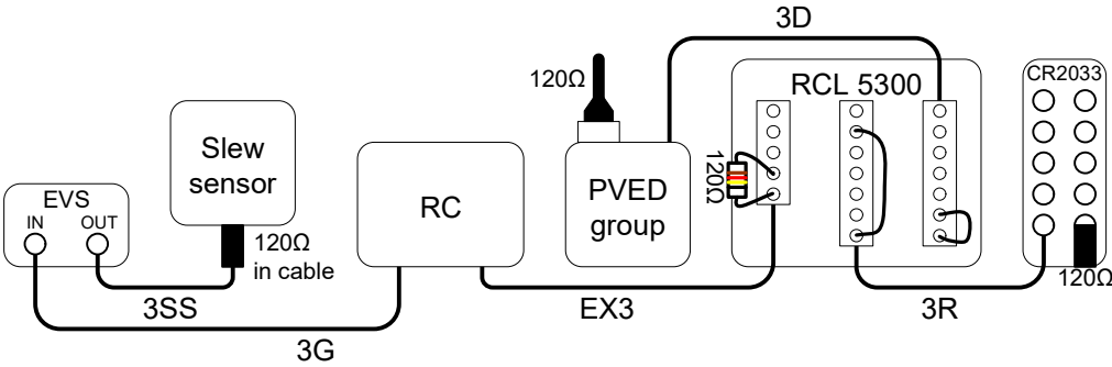
EVS Slew sensor RC, G2 CR2033
